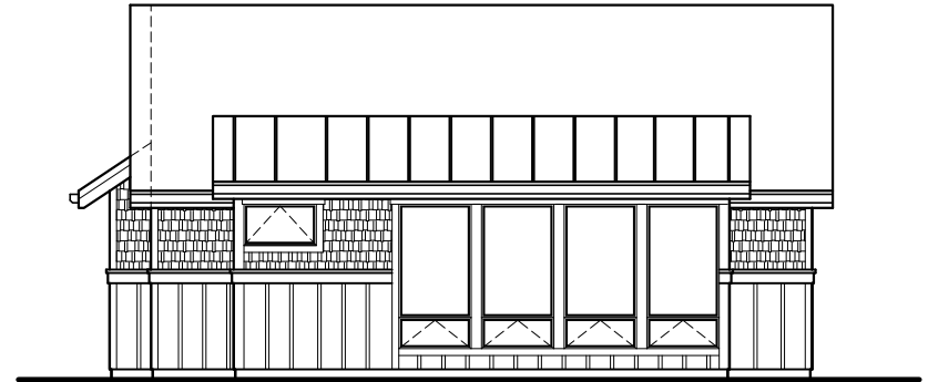
REAR ELEVATION
